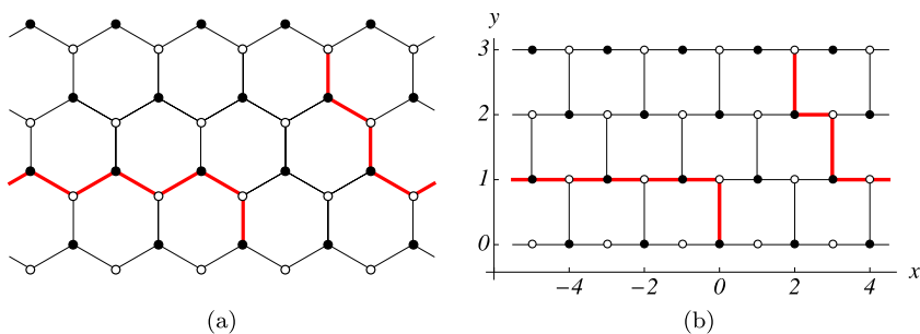
Fig. 4 (a) Cylindrical lattice domain of 5 \times 3 honeycombs with walk from lower to upper boundary. The highlighted curve represent some walk from the lower to the upper boundary. (b) Coordinate system for equivalent “brick wall” lattice
