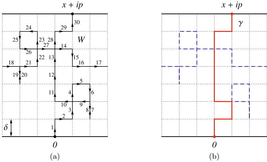
Fig. 2 Illustration of loop-erasure on the cylinder for a square lattice. (a) A Brownian excursion from z = 0 to the upper boundary y = p . (b) Loop-erasure of the same walk. Loops like (14, 15, \dots, 27) , winding around the cylinder for several times, may be erased
