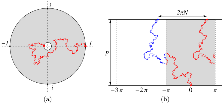
Fig. 1 (a) Illustration for SLE on an annulus \mathbb{A}_p from l to the target circle |z| = e^{-p} . (b) SLE on the cylinder and the covering space: the shaded region represents the cylinder, with sides x = -\pi and x = \pi identified. We obtain the covering space by periodic extension along the real axis. The endpoints on the cylinder and the covering space differ by 2\pi N where N denotes the winding number of the trace. The interfaces are samples of loop-erased random walks
